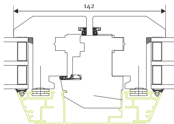
Central rullbåge
